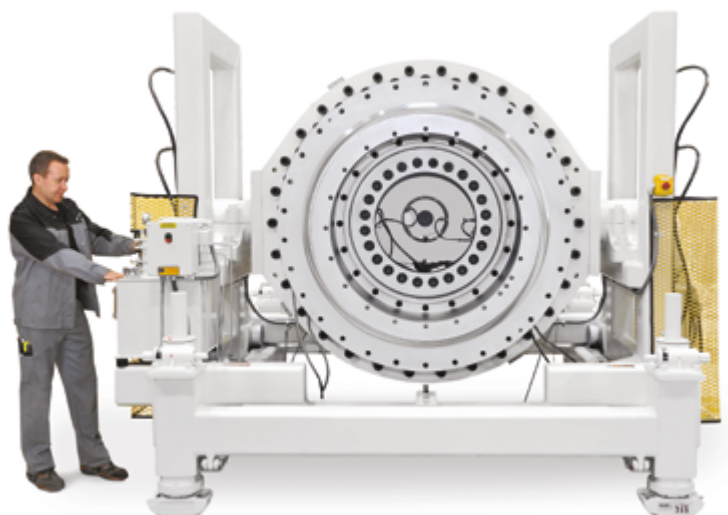
Spider double pipe head for 1,200 mm PVC pipe
