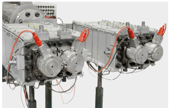
Spider 50-4 pipe die for quadruple strand extrusion of U-PVC pipes
