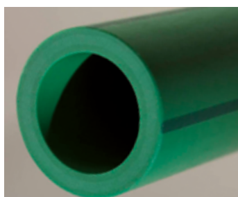
3-layer PP-R hot water pipes with glass fiber in the middle
