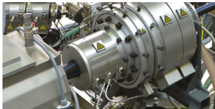
Pipe head for pipe-in-pipe extrusion
