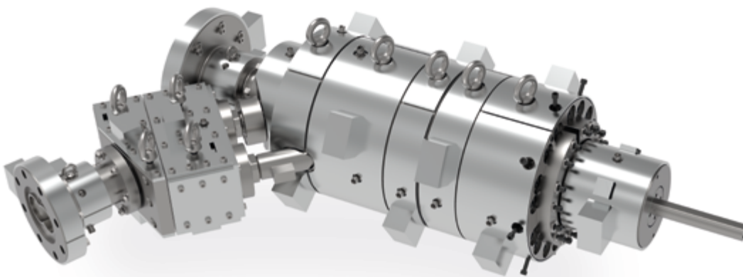
Spider pipe head for 3-layer PVC pipe
